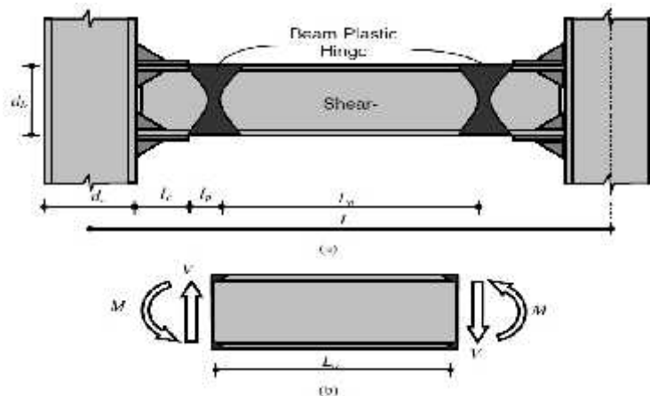
Gambar 3. Overstrength plastic hinge-based shear link[2]
